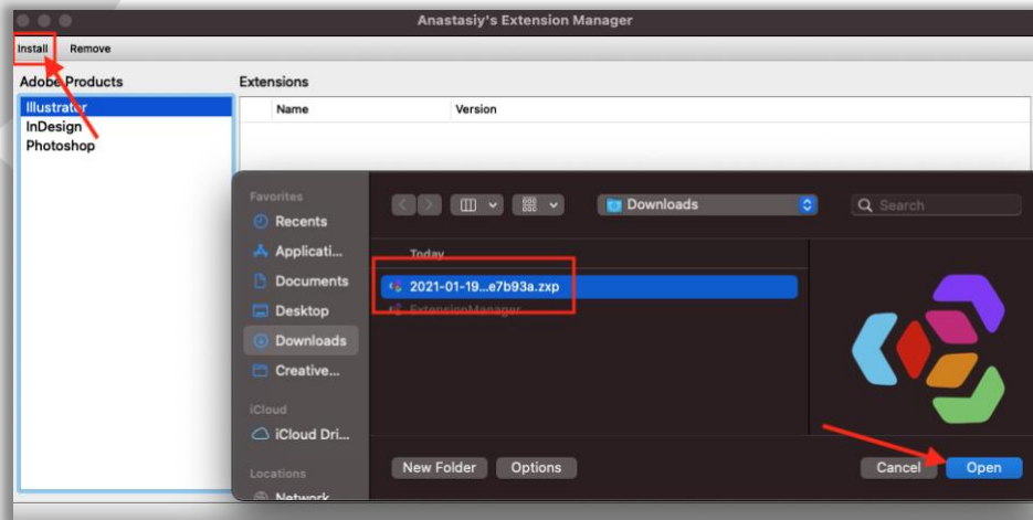
(Screenshot: Installationsvorgang)
